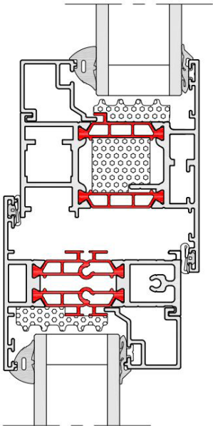
58BW CASEMENT HI MULLION
