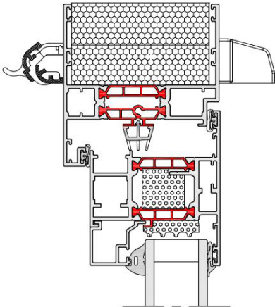
58BW CASEMENT HI HEAD
