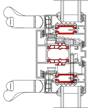
58BW ST FLUSH HI FRENCH CASEMENT
