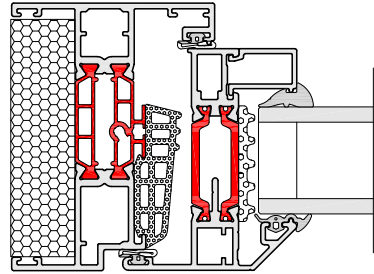
58BW ST FLUSH HI FRENCH CASEMENT
