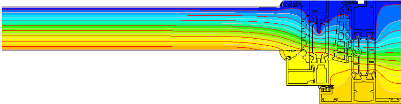
58BW ST FLUSH HI THERMAL PROFILE
