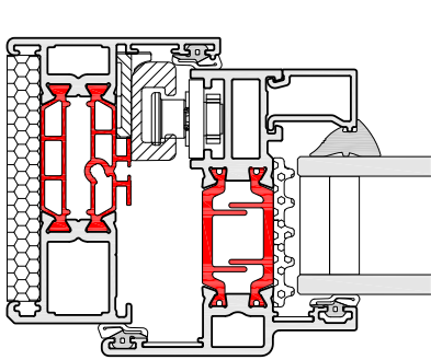
HERITAGE DOOR OPEN OUT LOCK JAMB
