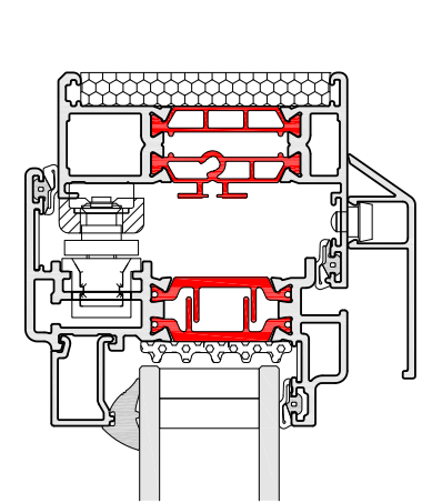
HERITAGE DOOR OPEN OUT CILL
